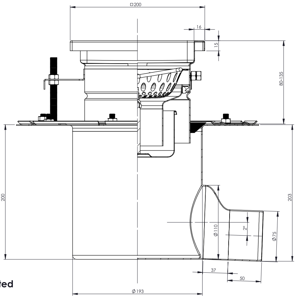
□ Krata / Mesh Anti-Slip H=30x2mm L15
